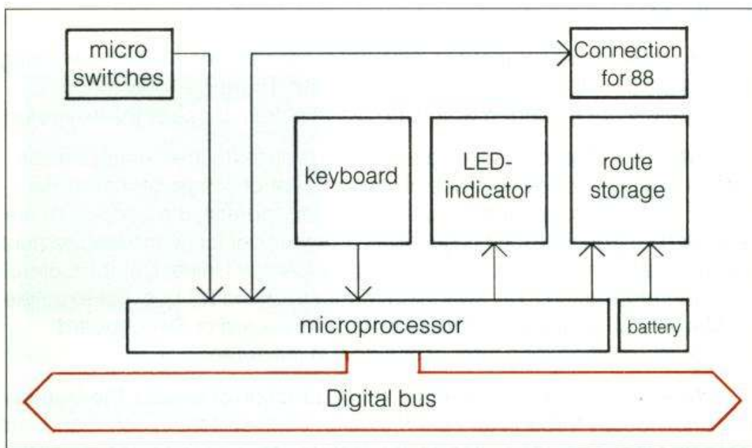
Block wiring diagram of the Memory
