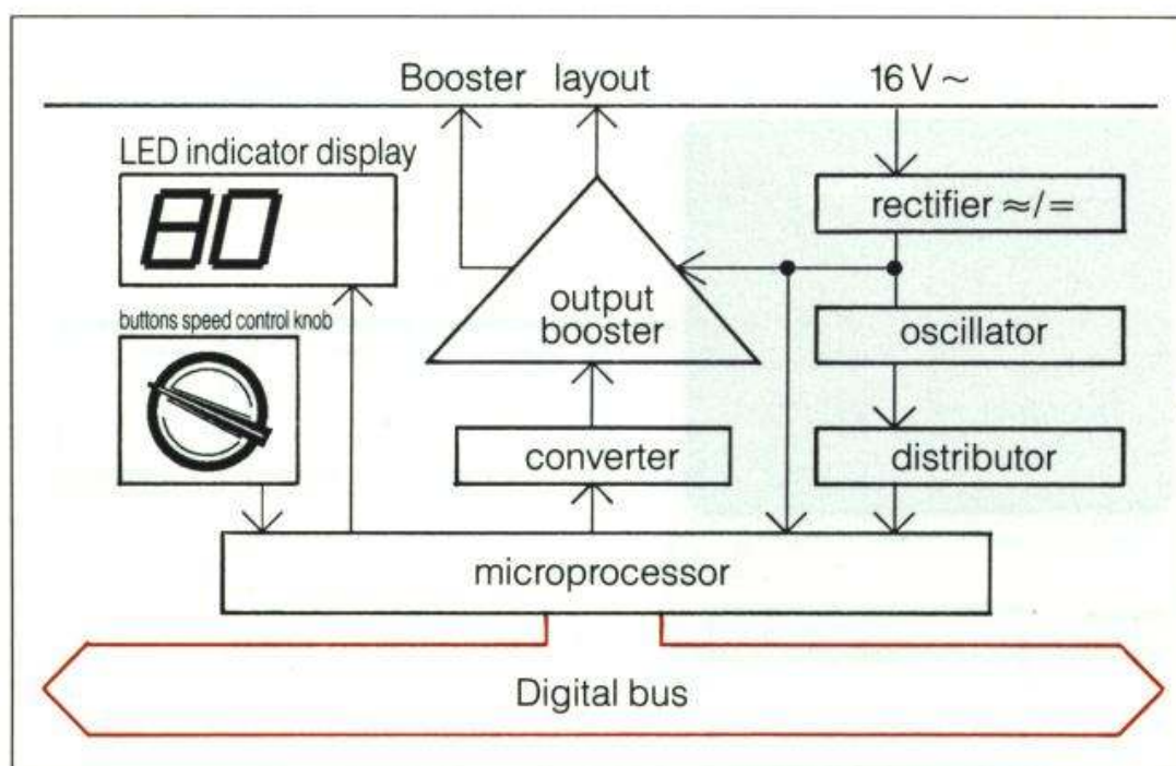
Block wiring diagram of the Central Control
