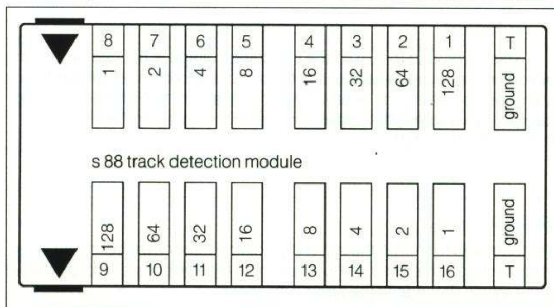
Relationship of the values to the contacts of the track detection module
