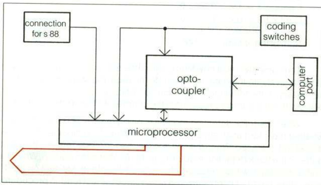
Block wiring diagram of the Interface
