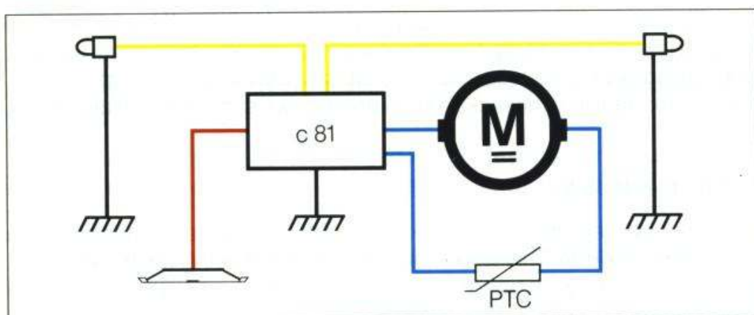
Wiring diagram for a c 81 decoder with headlights as the auxiliary function
