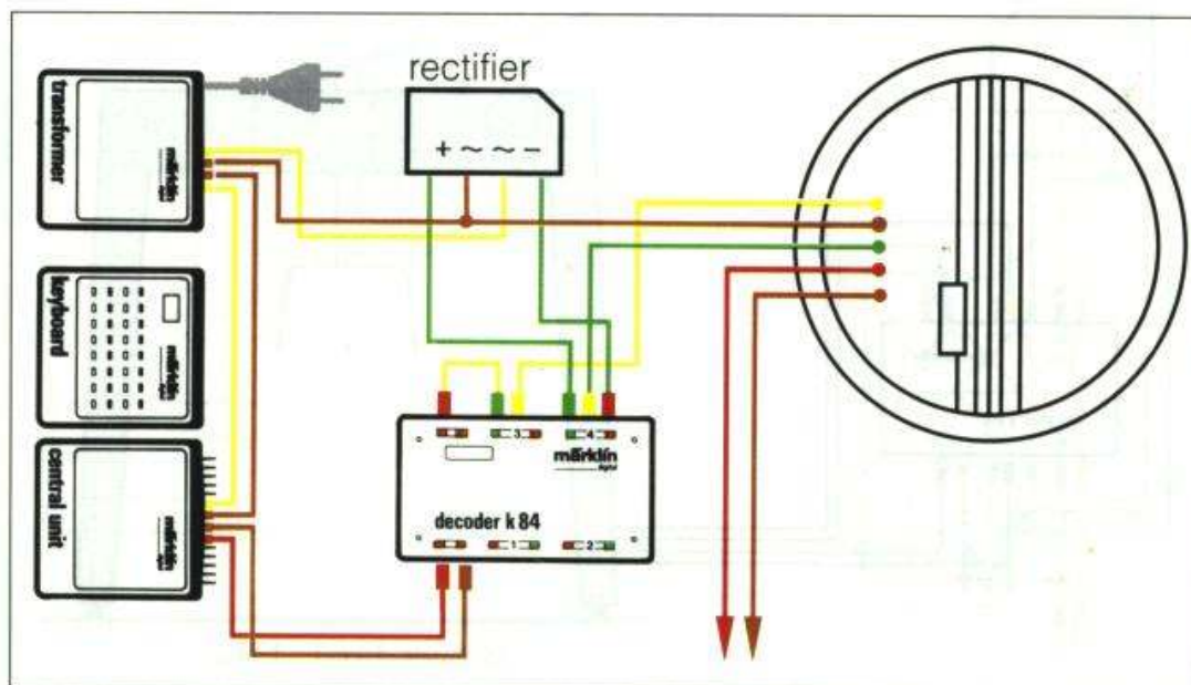
8998 Turntable controlled with the k 84 decoder
