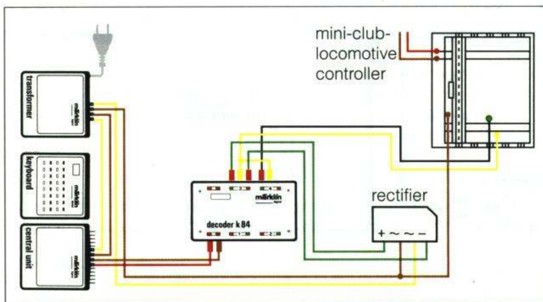
8994 Transfer table controlled with the k 84 decoder
