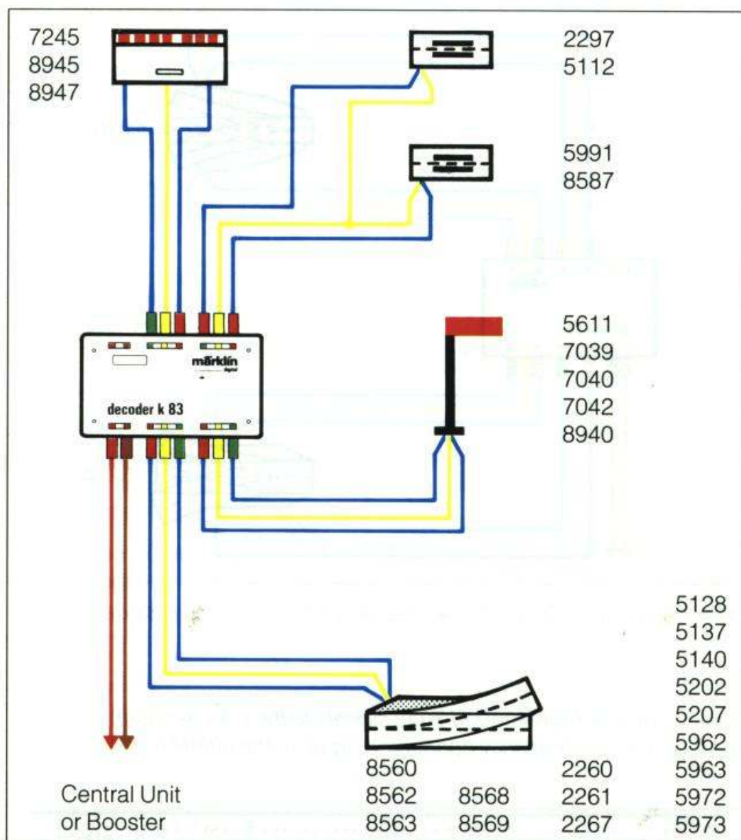
Basic hookup of solenoid accessories to the k 83 decoder
