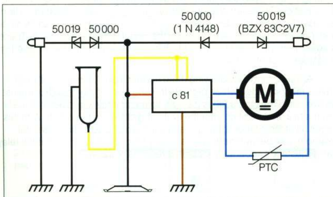
Separation of the headlights from the rest of the circuit using zenier diodes
