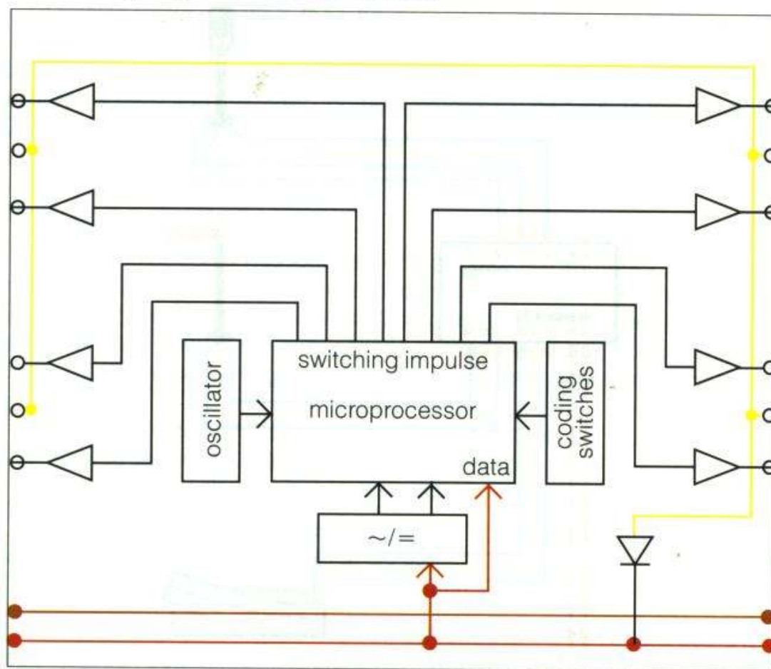
Block wiring diagram of the k 83 decoder
