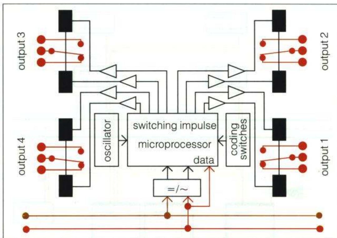
Block wiring diagram of the k 84 decoder
