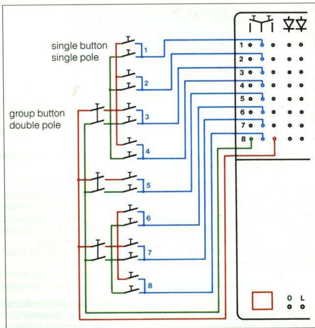
Hookup of individual buttons to the Switchboard
