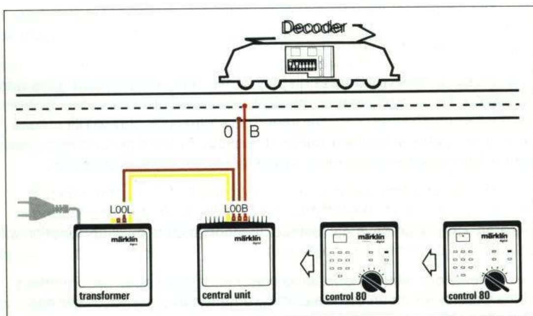
Plugging the Control 80 into the Central Unit
