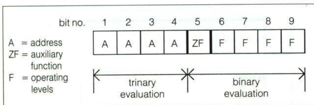
Data format for locomotive control
