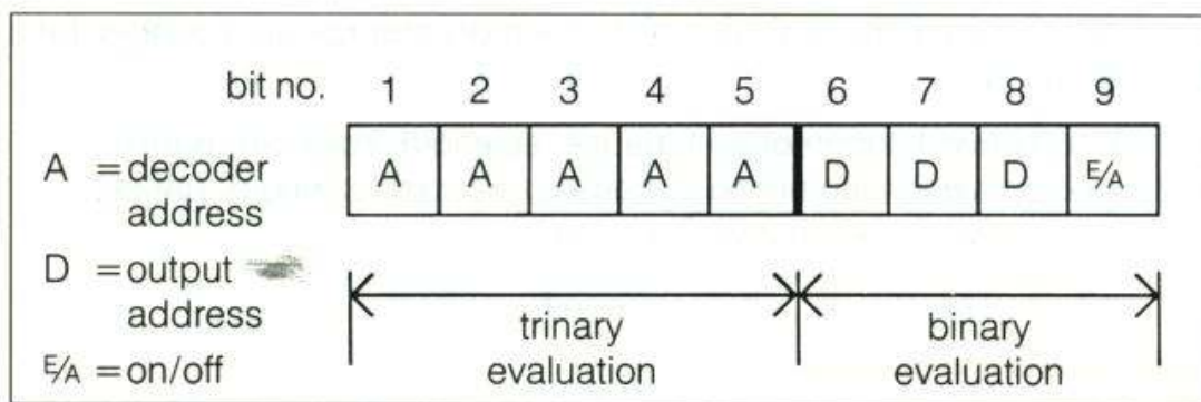
Data format for switching solenoid accessories
