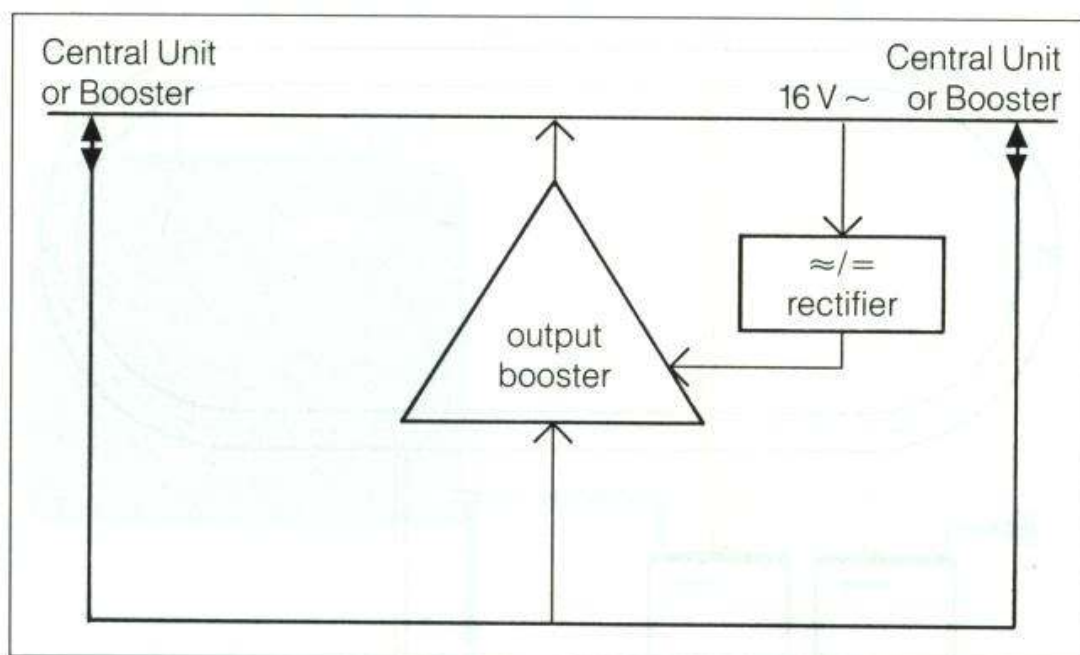
Block wiring diagram of the Booster
