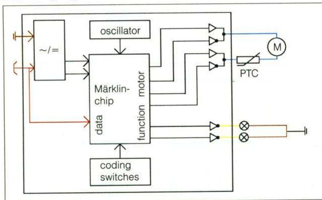
Block wiring diagram of the c 81 decoder
