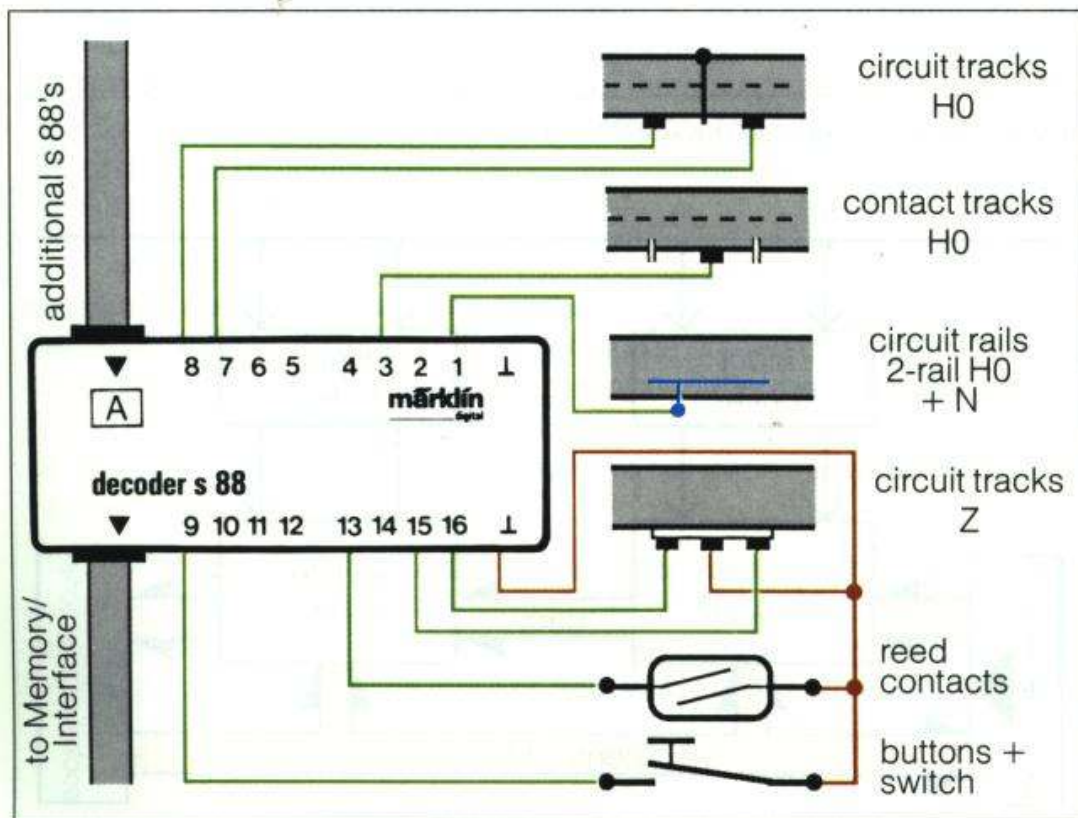
Hooking up the track detection contacts to the s 88 track detection module
