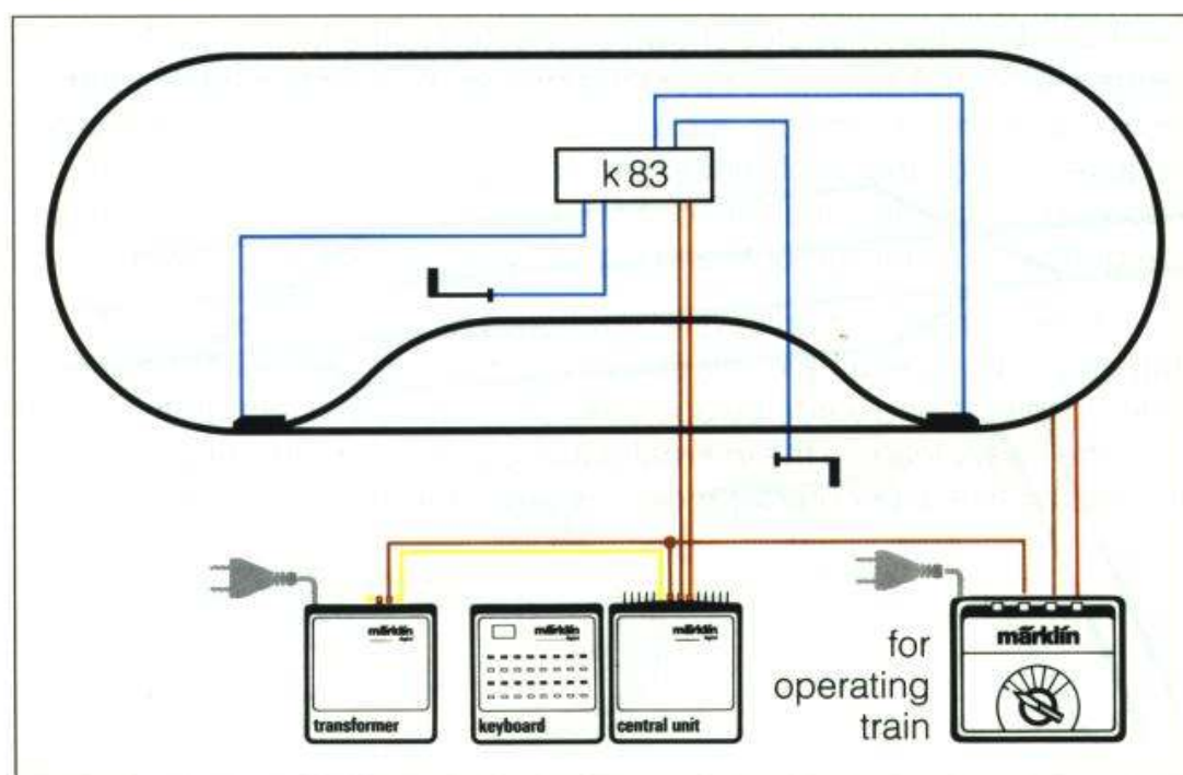
Basic setup for switching turnouts and signals
