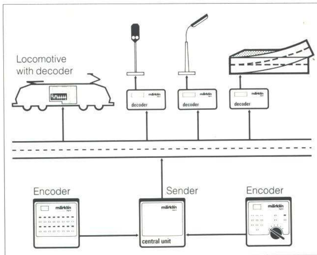
Control of a model railroad with the Märklin Digital system (diagram)
