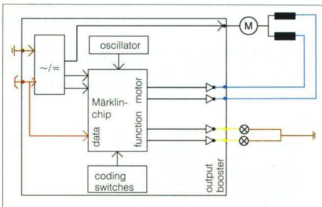
Block wiring diagram of the c 80 decoder
