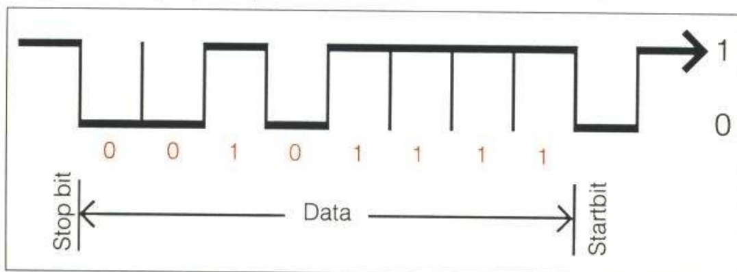
Diagram of a byte (8 bits)
