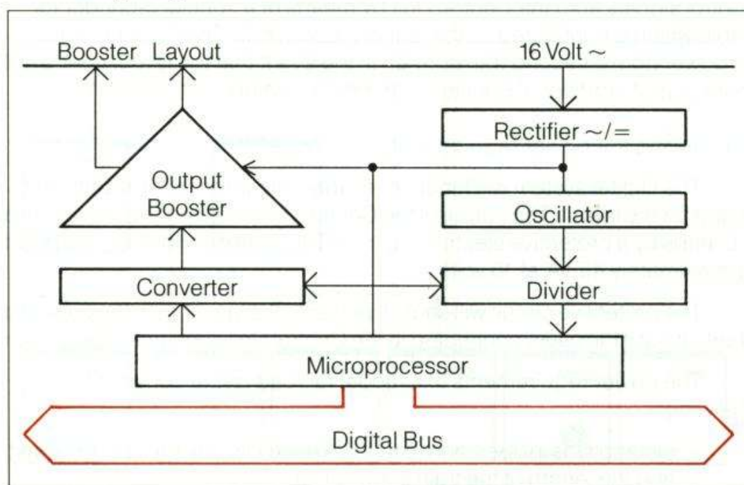
Block wiring diagram of the Central Unit
