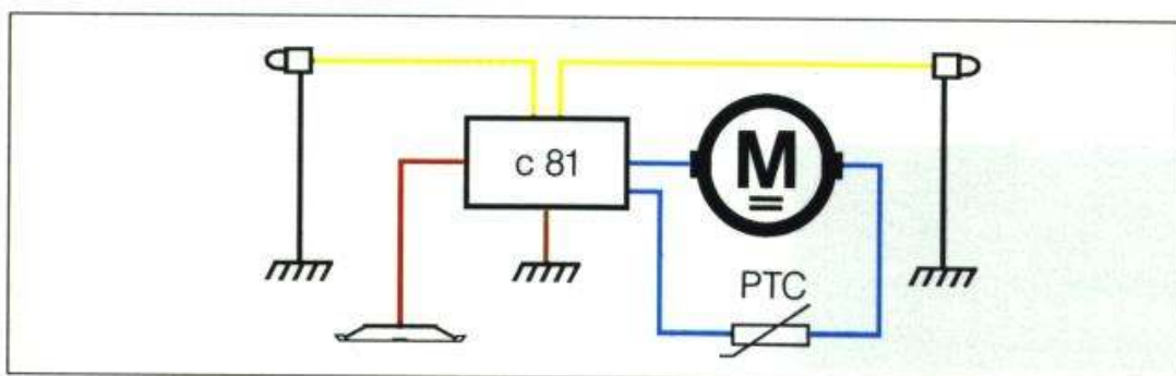
Hookup for the c 81 decoder
