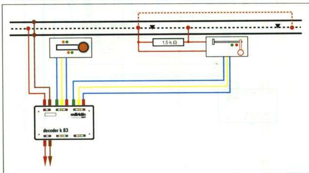
Wiring diagram for a 7039 signal with a 7036 distant signal and train control capabilities
