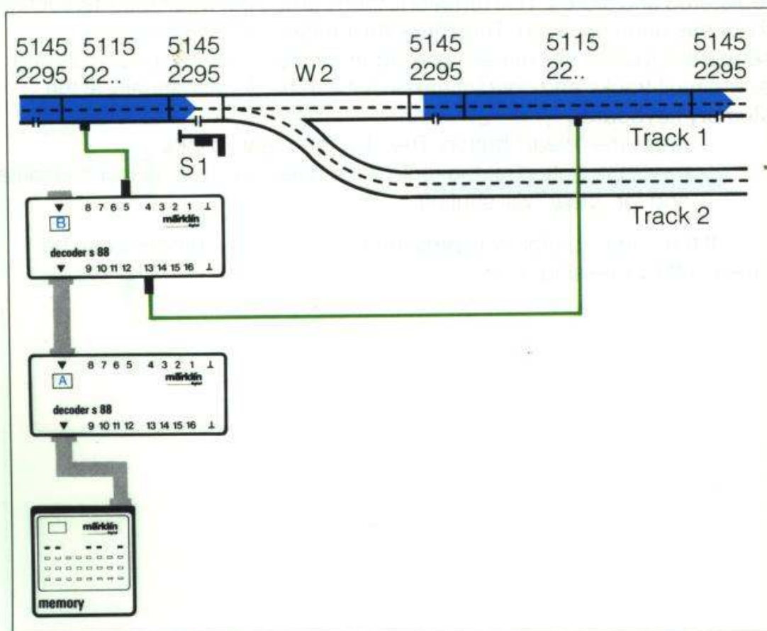
A sample station layout
