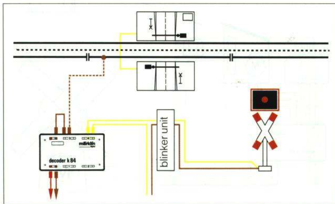
Hookup for the 7192, 7292 and 7592 crossing gates
