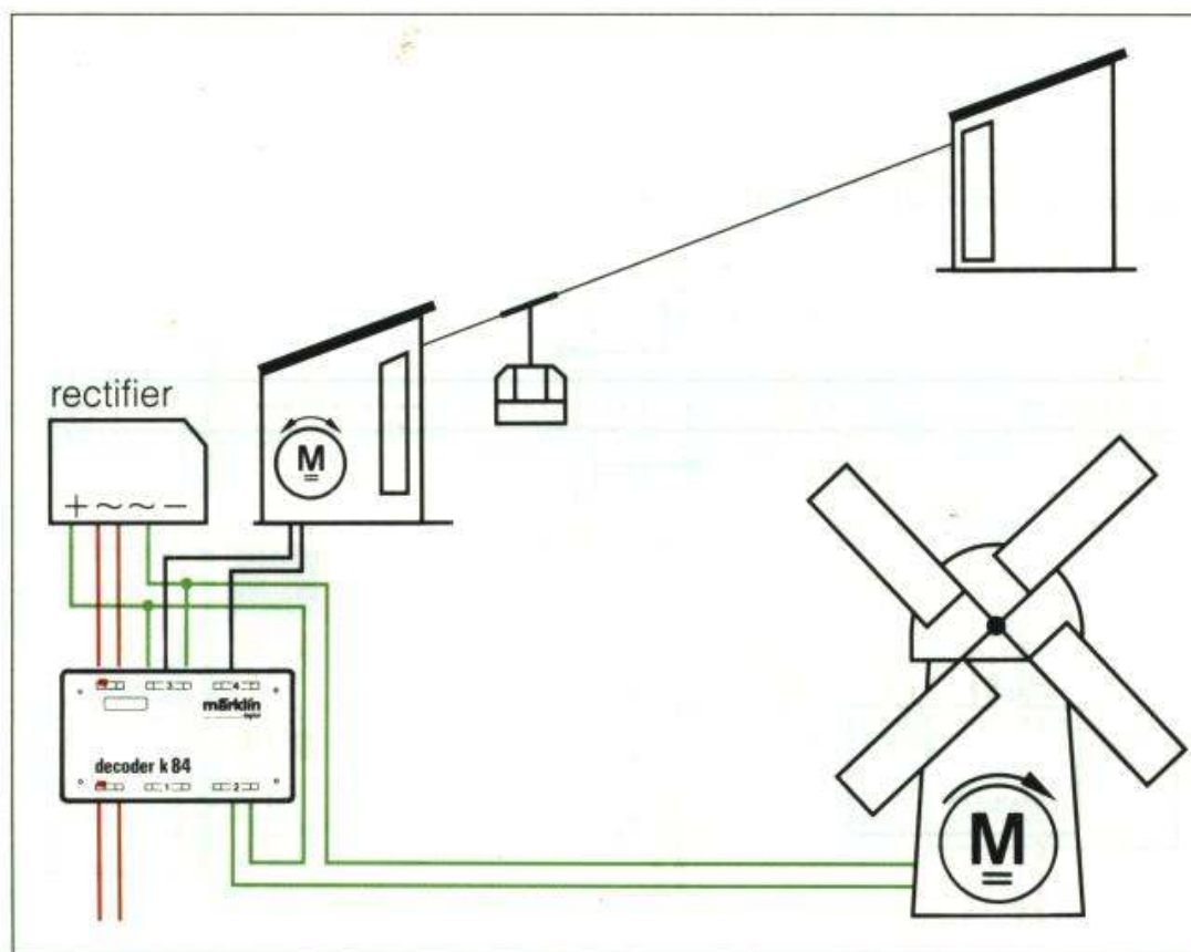
Hookup for a cable car, windmill and lighting installation to the k 84 decoder
