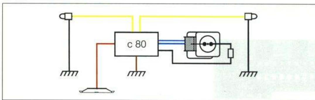
Hookup for the c 80 decoder
