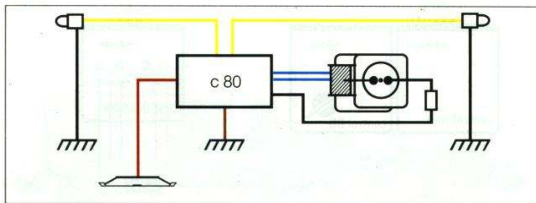
Wiring diagram for the c 80 decoder with headlights as the auxiliary function
