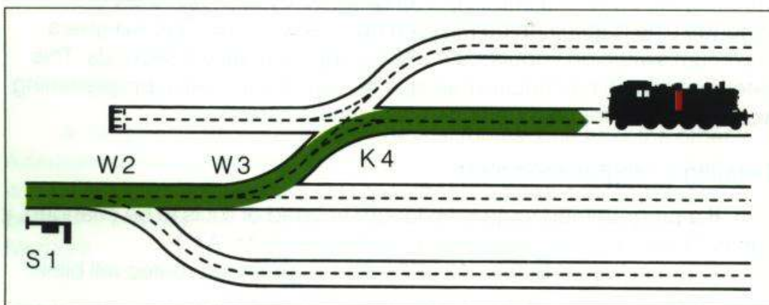
A section of a sample station layout
