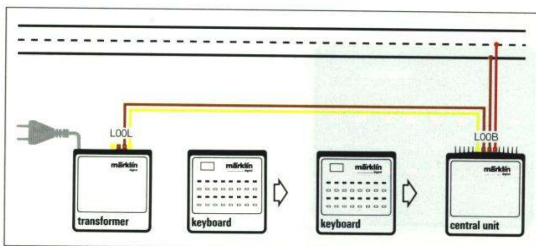
Plugging the Keyboard into the Central Unit
