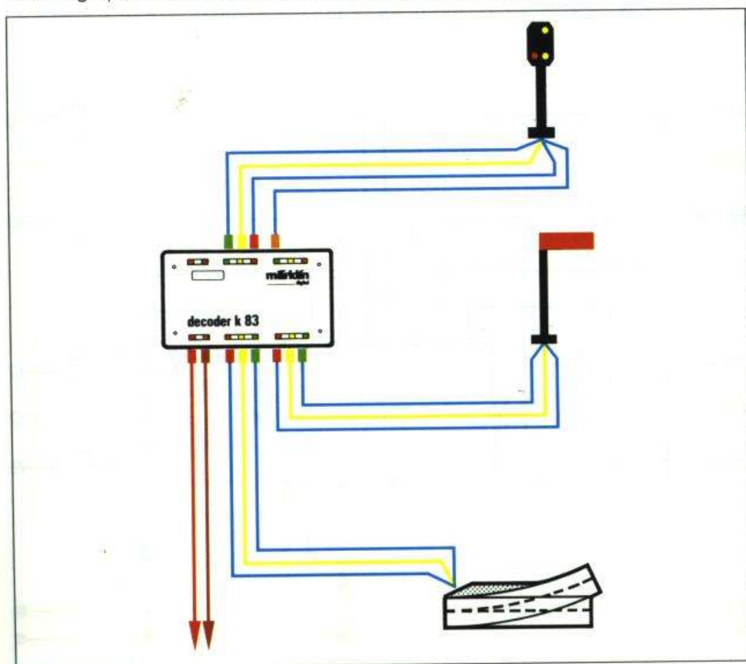
Hooking up turnouts and signals to the k 83 decoder
